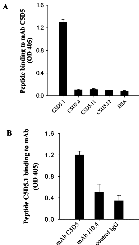
FIGURE 1. Peptide C5D5.1 binds directly and specifically to mAb C5D5. A , As detailed in Materials and Methods , binding of mAb C5D5 to microtiter wells coated with peptide C5D5.1 (oxidized) or control peptides C5D5.4, C5D5.11 (oxidized), and C5D5.12 (oxidized) is shown. B , Peptide C5D5.1 (oxidized) specifically binds to mAb C5D5 but not control mouse IgG. The data represent the mean and SD of triplicate wells per condition in one of three experiments.
