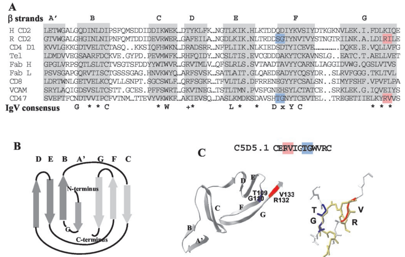
FIGURE 5. A putative SIRP \alpha binding domain on the CD47 protein surface. A , The CD47 IgV domain sequence is aligned with other IgV superfamily members based on consensus primary sequence patterns (10): +, basic amino acids; *, hydrophobic amino acids. Structurally conserved \beta strands (A' to G) are shaded. B , The conserved “Greek Key” topology of IgV structure (10) containing two layers of antiparallel \beta -strand sheets. Note that the sheet containing strands G, F, and C contains residues on the protein surface. C , Protein modeling of peptide C5D5.1. Left , Modeling of CD47 extracellular IgV domain based on the IgV structure of CD2 (ribbon model) (39). The putative binding site containing residues RV and TG is colored (red and blue, respectively) and illustrates the proximity of these residues on the protein surface. Right , Overlaying the entire C5D5.1 sequence (gold) onto residues TG (blue) and RV (red) on F and G strands. Protein structural modeling was performed using The Deep View/Swiss-PDB Viewer version 3.7 (GlaxoSmith-Kline, Research Triangle Park, NC).
