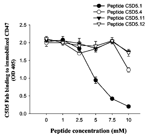
FIGURE 2. Inhibition of CD47-C5D5 Fab binding by peptide C5D5.1. Microtiter plate wells were coated with purified CD47 (from human PMN) for 2 h. After blocking, C5D5 Fab (1 \mu g/ml) was added into wells without or with increasing amounts of peptide C5D5.1 (●), control peptides C5D5.4 (○), C5D5.11 (▲), or C5D5.12 (△). Peptides C5D5.1, C5D5.11, and C5D5.12 were oxidized. Binding of C5D5 Fab to CD47 was detected by a peroxidase-conjugated secondary Ab. The data represent the mean \pm SD of triplicate wells per condition in one of three experiments.
