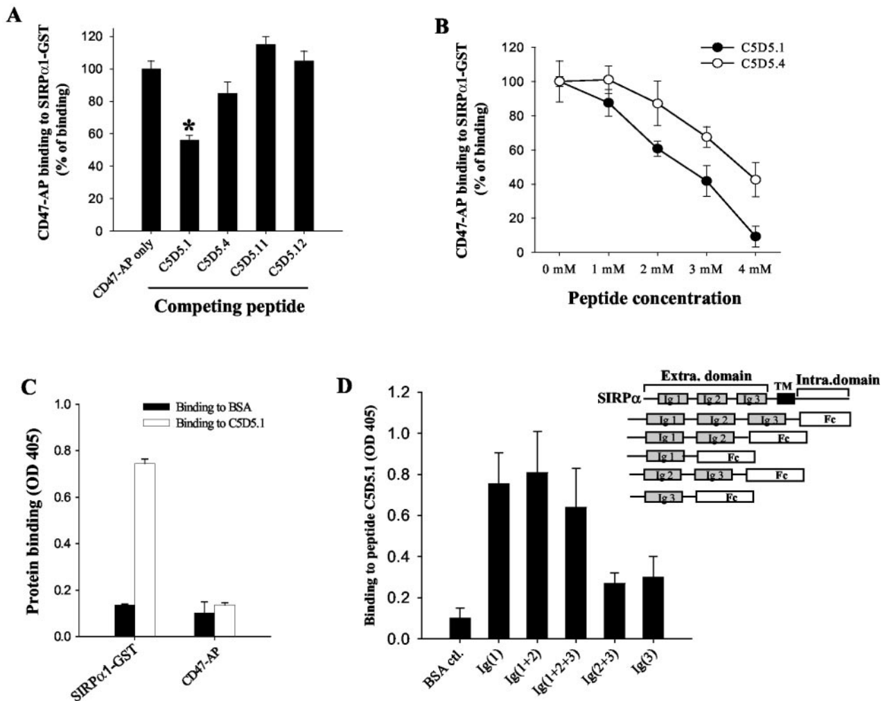
FIGURE 4. A, Inhibitory effects of peptide C5D5.1 on CD47-SIRP \alpha binding. Microtiter plates were coated with SIRP \alpha 1-GST fusion protein (2 \mu g/ml). After blocking, CD47-AP was added in the absence or presence of synthetic peptide C5D5.1, control peptides C5D5.4, C5D5.11, or C5D5.12 (used as 2 mM each). After washing, binding of CD47-AP to SIRP \alpha 1-GST was detected by assay of AP (*, p < 0.01 ). B, Dose-dependent inhibition of CD47-SIRP \alpha 1 binding by adding increasing amounts of peptide C5D5.1 and control peptide C5D5.4 as in A. C, Peptide C5D5.1 binds directly to SIRP \alpha 1-GST. Microtiter plates were coated with 2 mM peptide C5D5.1 or 1% BSA. After blocking, wells were incubated with either SIRP \alpha 1-GST or CD47-AP (5 \mu g/ml) and binding was detected by a goat anti-GST Ab (for SIRP \alpha 1-GST) or by assay of AP (for CD47-AP). D, Peptide C5D5.1 binds to the membrane distal Ig loop (Ig1) of SIRP \alpha 1. Recombinant Fc fusion proteins containing different Ig loop(s) of SIRP \alpha 1 extracellular domain were generated as detailed in Materials and Methods and illustrated as in the figure inset (Fig 4D, inset ). Binding of these Fc fusion proteins to immobilized peptide C5D5.1 was measured by a peroxidase conjugated anti-rabbit IgG. Peptides used including C5D5.1, C5D5.11, and C5D5.12 were oxidized. All data represent the mean \pm SD of triplicate wells per condition in one of three experiments.
